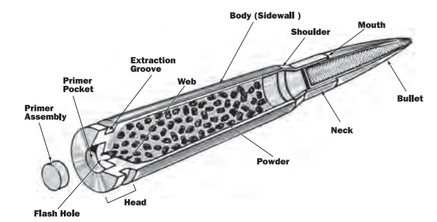
Remove spent primer and size case
